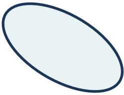
Ellipse: setRotation
